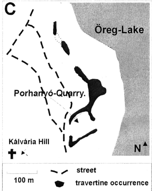
1. The travertine occurrences at the Öreg-Lake (Tata) (modified after the geologic map of Gyalog 2003) and location of the Kőpíte-Hill (travertine cone?)
