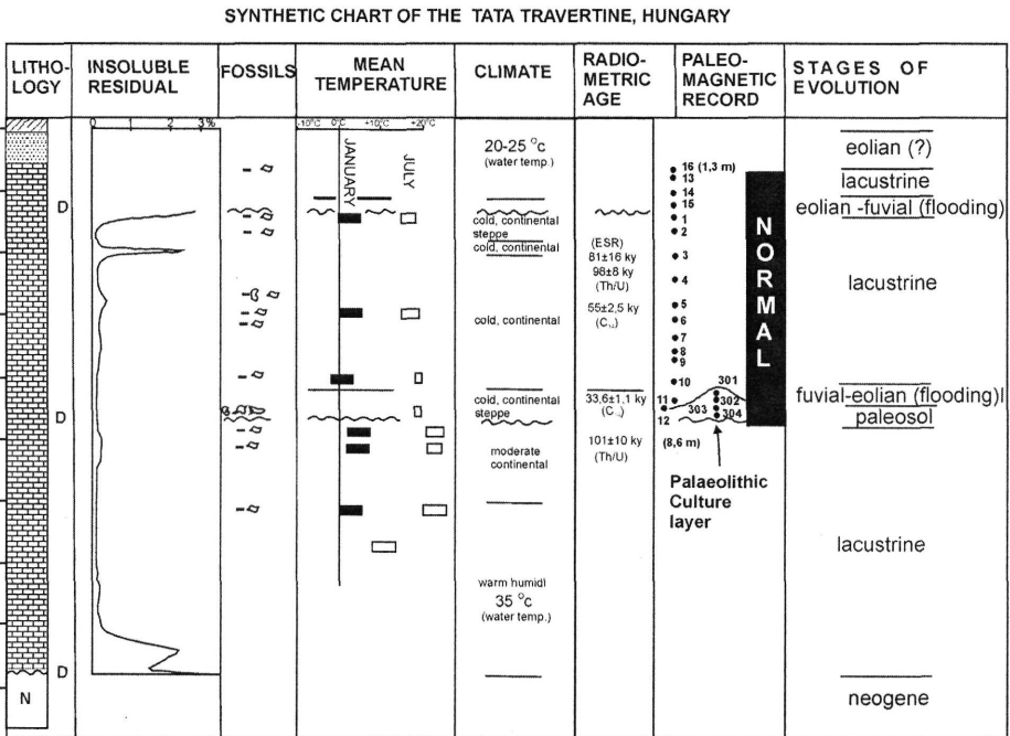
12. Synthetic chart of Tata freshwater limestone (chronology and palaeoenvironmental relation)
