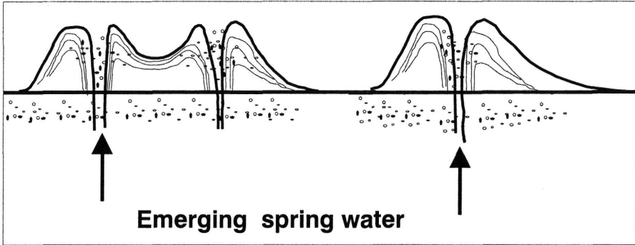
11. Sketch of the carbonate vents (with quartz grains deriving from the Pannon siliclastic bedrock) occurring in the quarry
