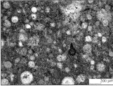
1. Radiolarite (1) thin section, iN 4x objective
