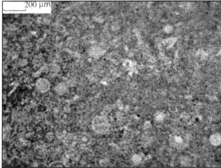
5. Radiolarite (2) thin section, iN 4x objective
