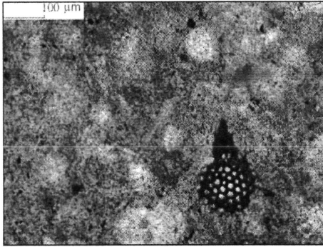
3. Radiolarite (1) thin section, XN 10x objective
