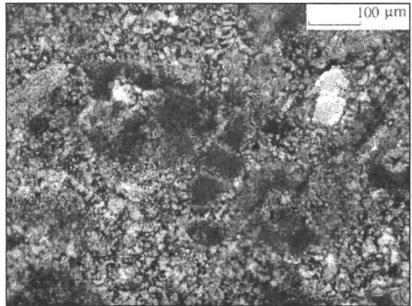
6. Spongiolite thin section, XN 10x objective with sponge spicules and Foraminifera
