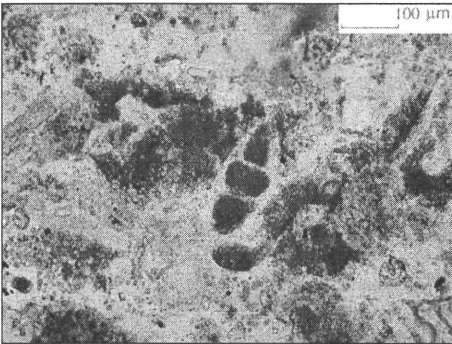
5. Spongiolite thin section, 1N 10x objective with sponge spicules and Foraminifera
