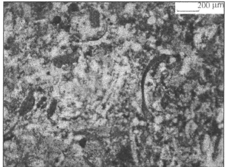
4. Spongiolite thin section, XN 4x objective with sponge spicules
