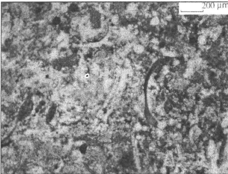
3. Spongiolite thin section, 1N 4x objective with sponge spicules
