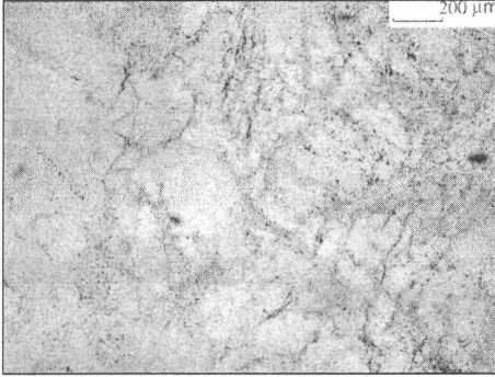
1. Quartzite thin section, 1N 4x objective
